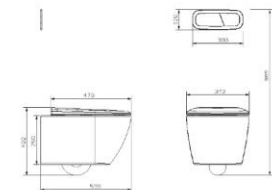
SKY-WT Wall Hung Toilet Size: 479x373x402mm Customized
