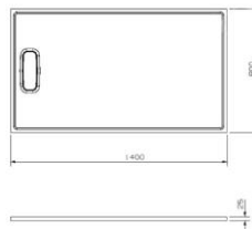
SKY-ST Shower Tray Customized
