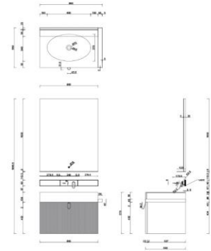
ETCB-S+ Cabinet
